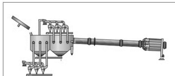
Figure 21. Lepol Kiln
