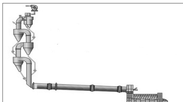
Figure 22 – cyclone preheater
